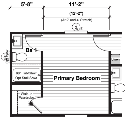
Option Bedroom / Bath Layout
