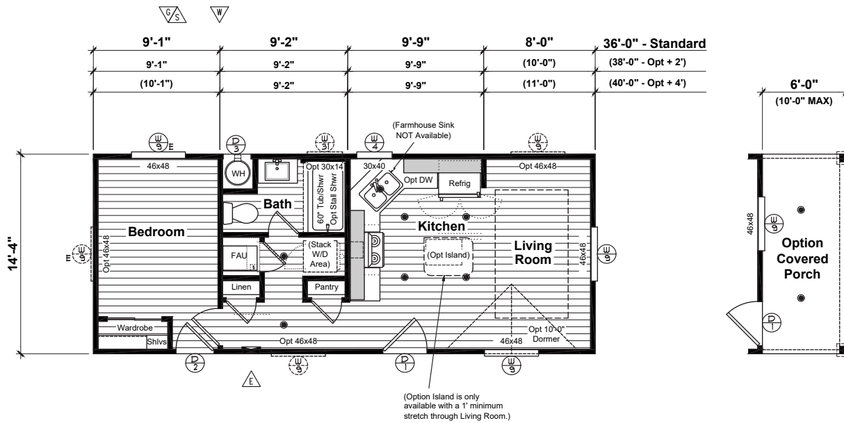
Model 1436-1A 1 Bedroom, 1 Bath - 516 Sq. Ft.
